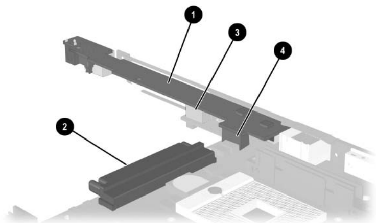
Figure 5-27. Proper Handling of the I/O Interface Board on Evo Notebook N620c, N610c, and N610v Models
