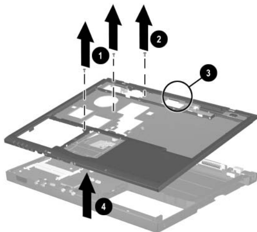
Figure 5-21. Removing the Top Cover
