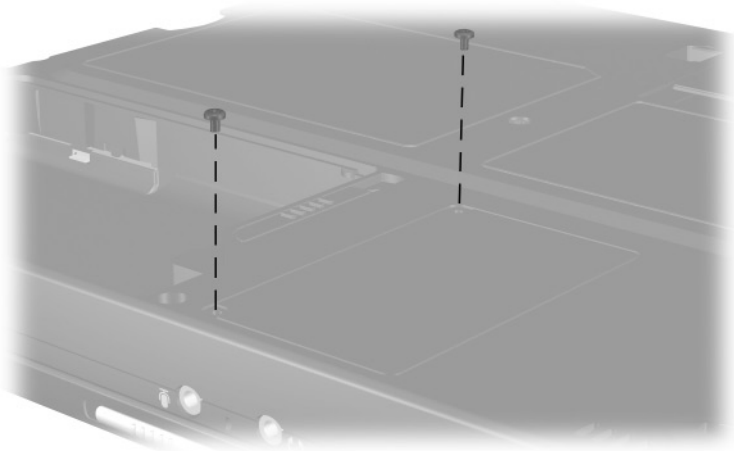
Figure C-3. PM2.5 × 5.0 Screw Location
