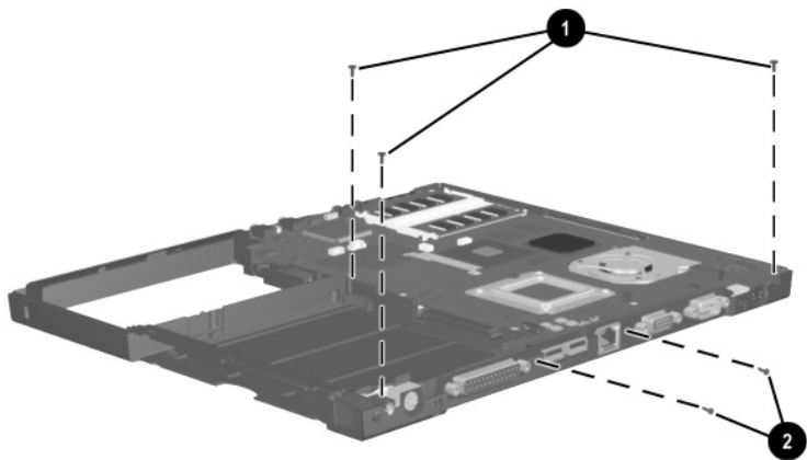
Figure C-9. M2.5 × 5.0 Screw Locations
