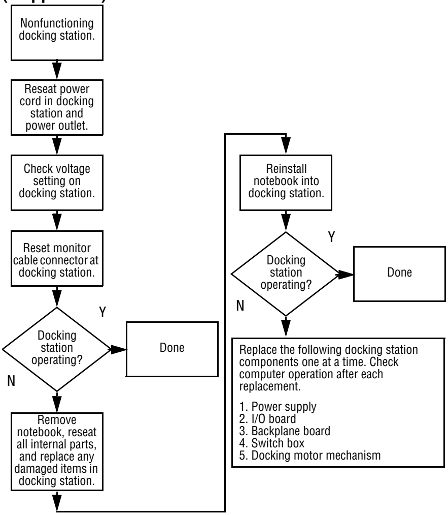
Flowchart 2.8 - Nonfunctioning Docking Station (if applicable)
