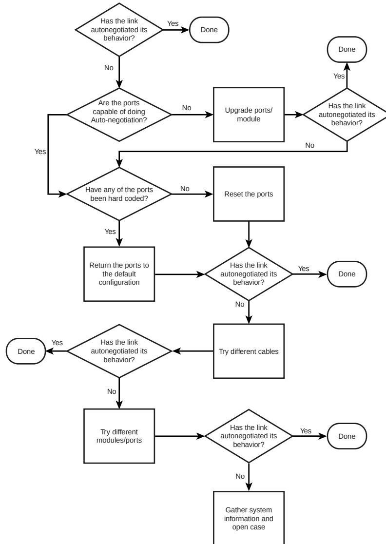
Figure 23-2 Troubleshooting Ethernet Autonegotiation
