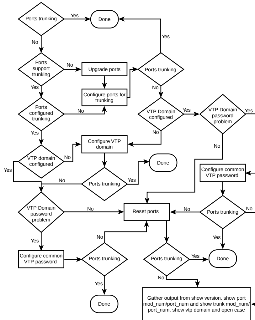
Figure 23-4 Troubleshooting ISL Trunking on Catalyst 5000 and 6000 Family Switches
